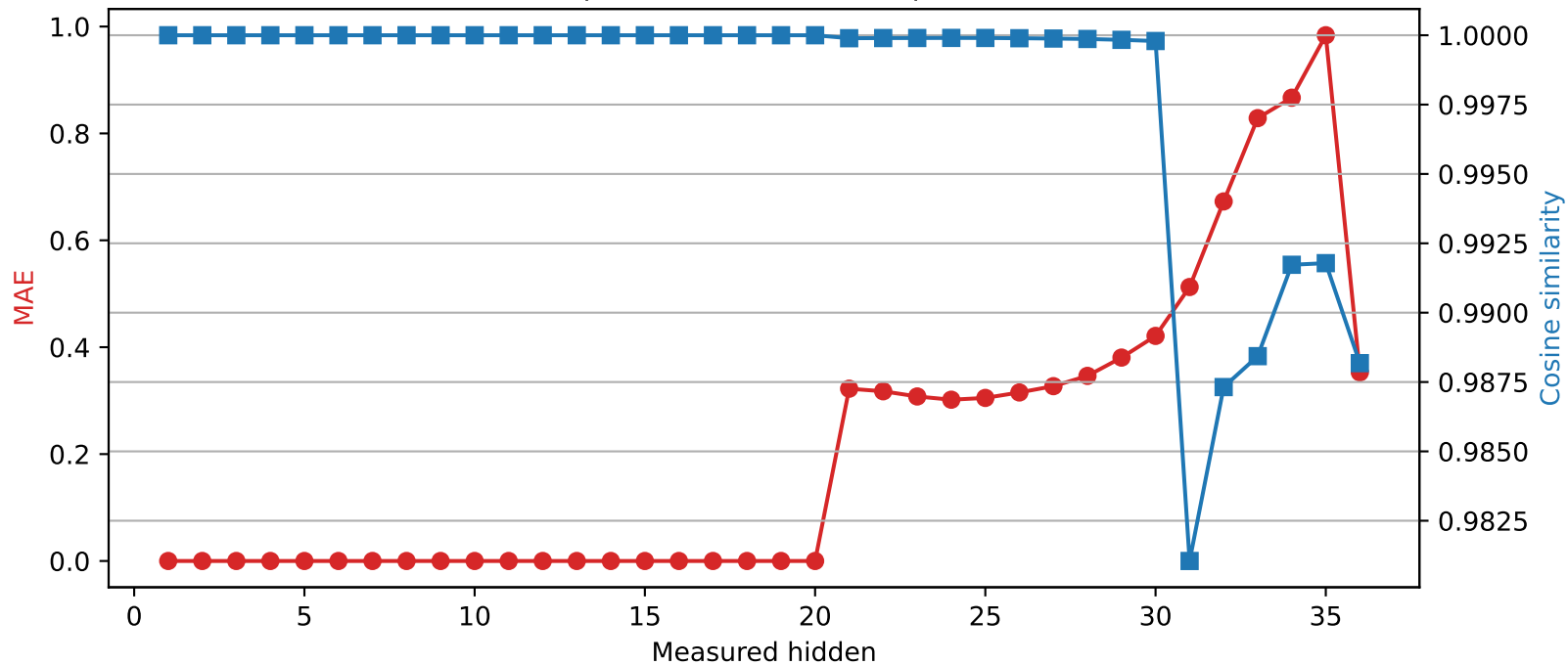
Qwen2.5-3B | Quantized layer 20 | float16 → int4
