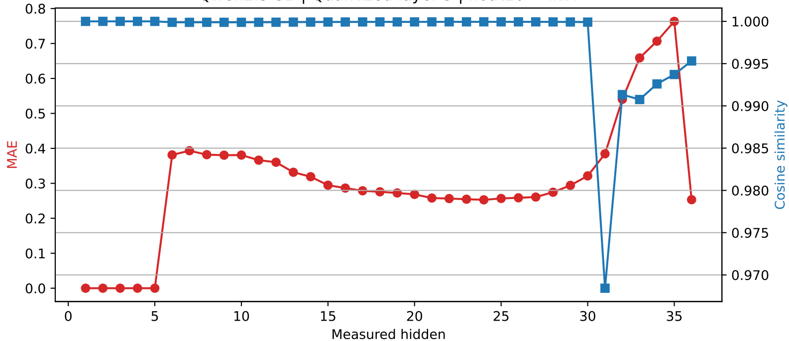
Qwen2.5-3B | Quantized layer 5 | float16 \rightarrow int4
