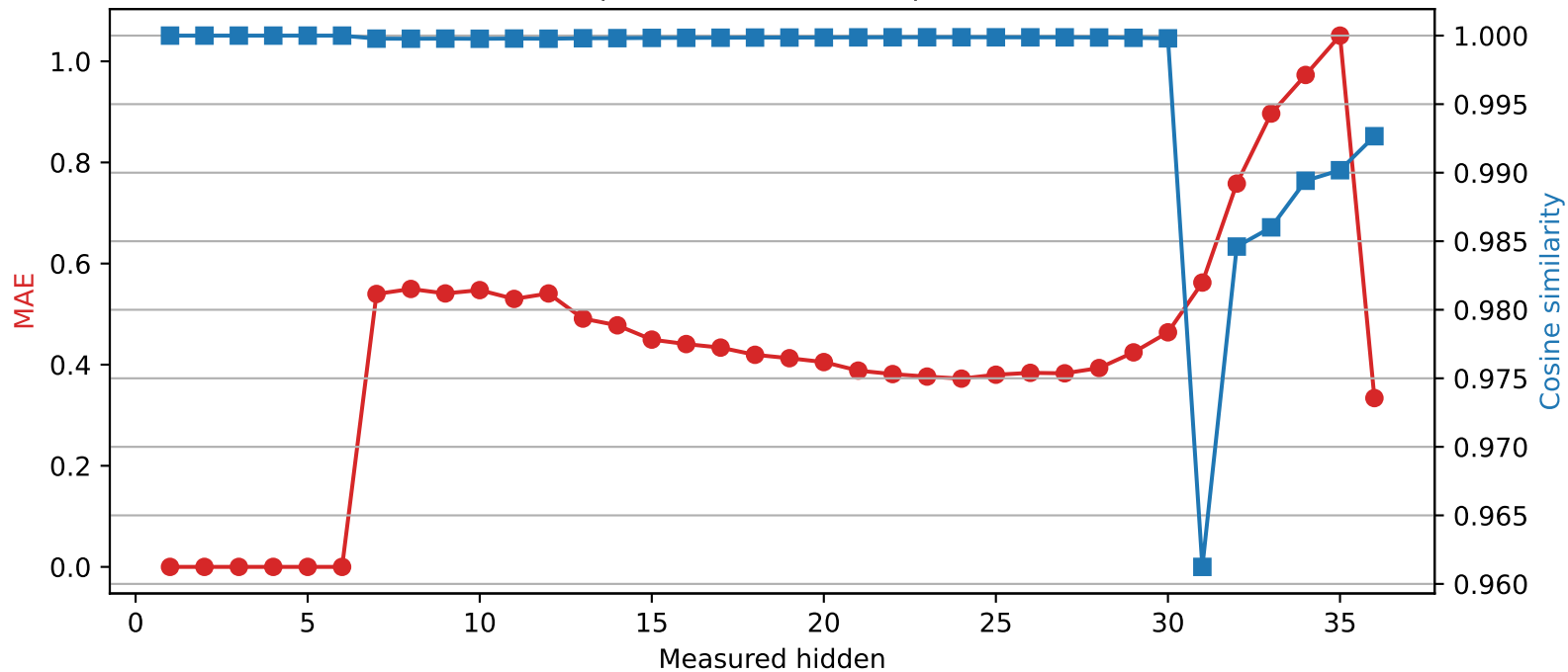
Qwen2.5-3B | Quantized layer 6 | float16 → int4
