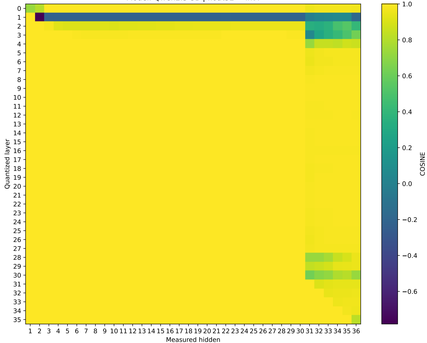
Model: Qwen2.5-3B | float32 \rightarrow int4
