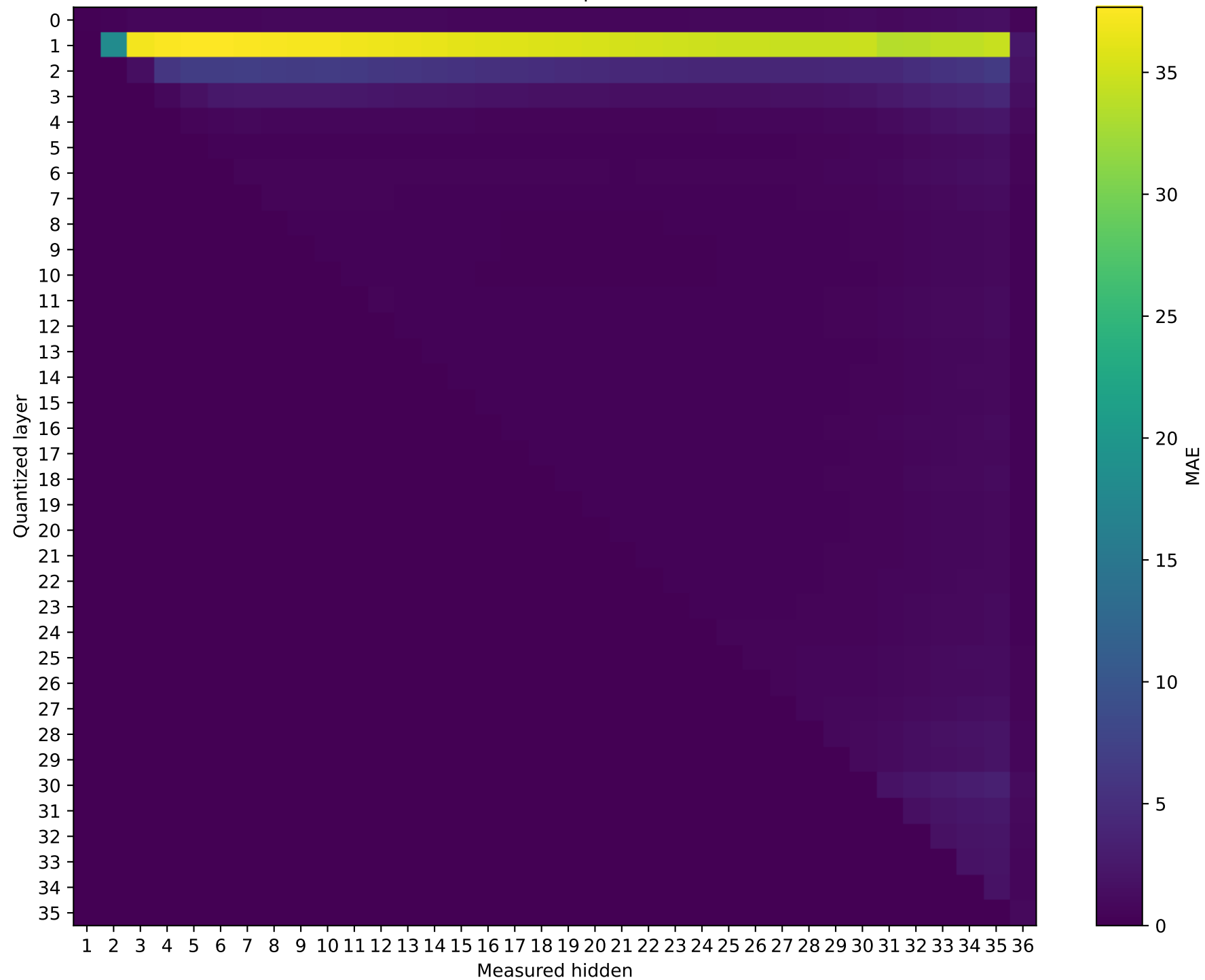
Model: Qwen2.5-3B | float32 \rightarrow int4
