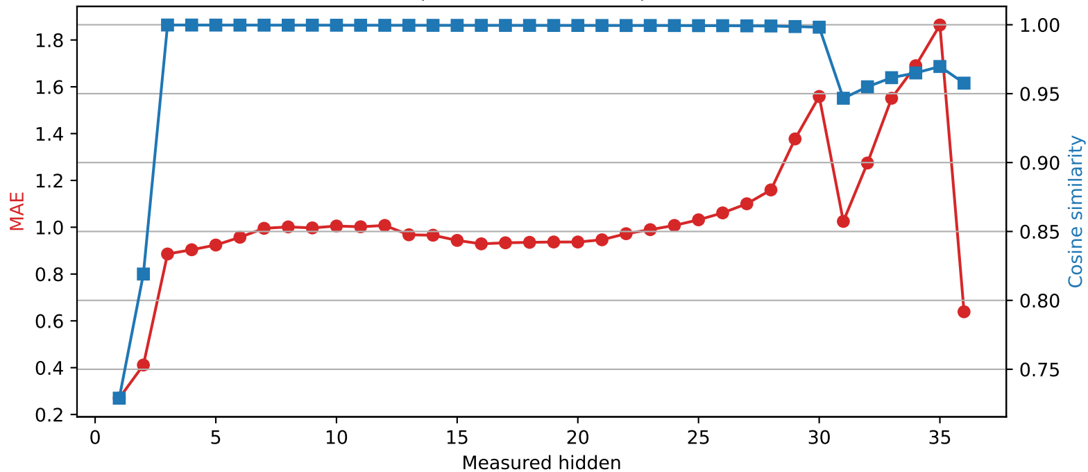
Qwen2.5-3B | Quantized layer 0 | float32 → int4
