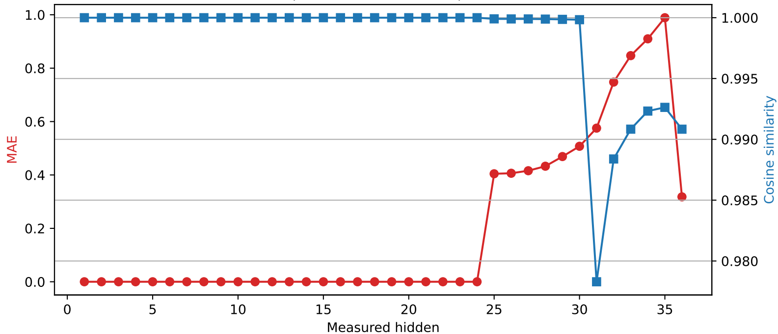
Qwen2.5-3B | Quantized layer 24 | float32 → int4
