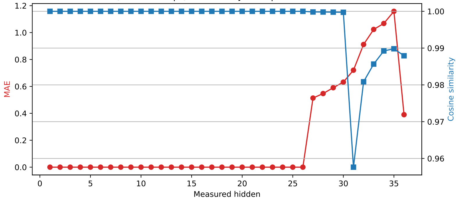
Qwen2.5-3B | Quantized layer 26 | float32 → int4
