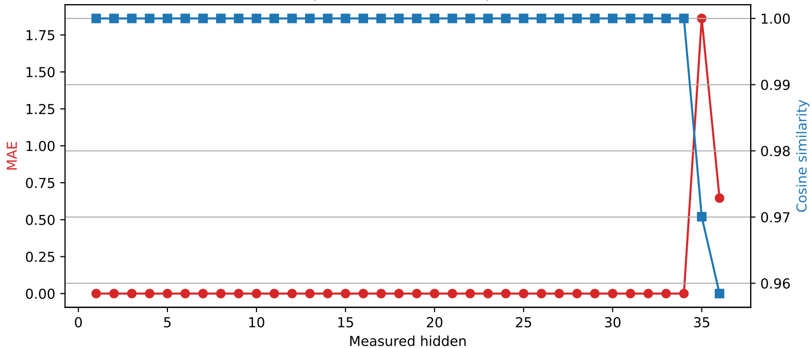
Qwen2.5-3B | Quantized layer 34 | float32 \rightarrow int4
