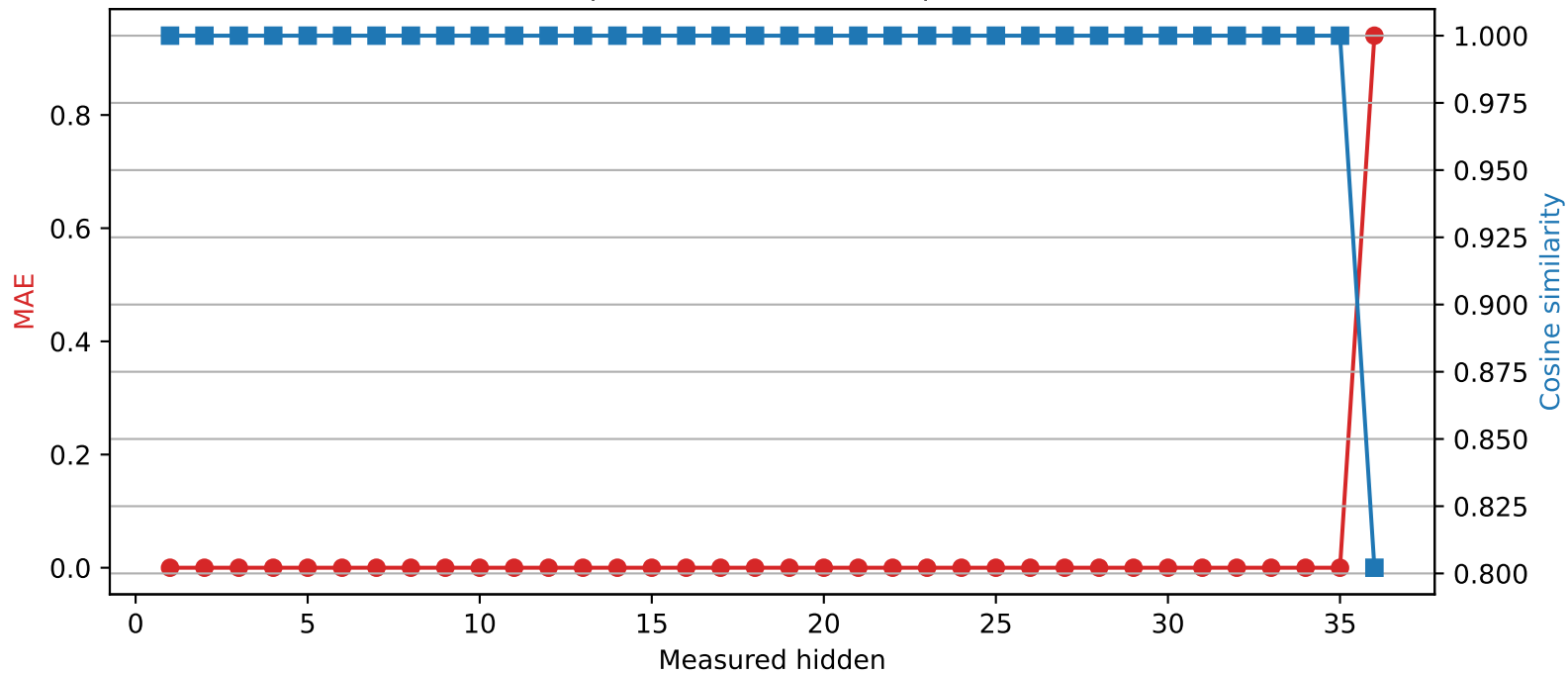
Qwen2.5-3B | Quantized layer 35 | float32 → int4
