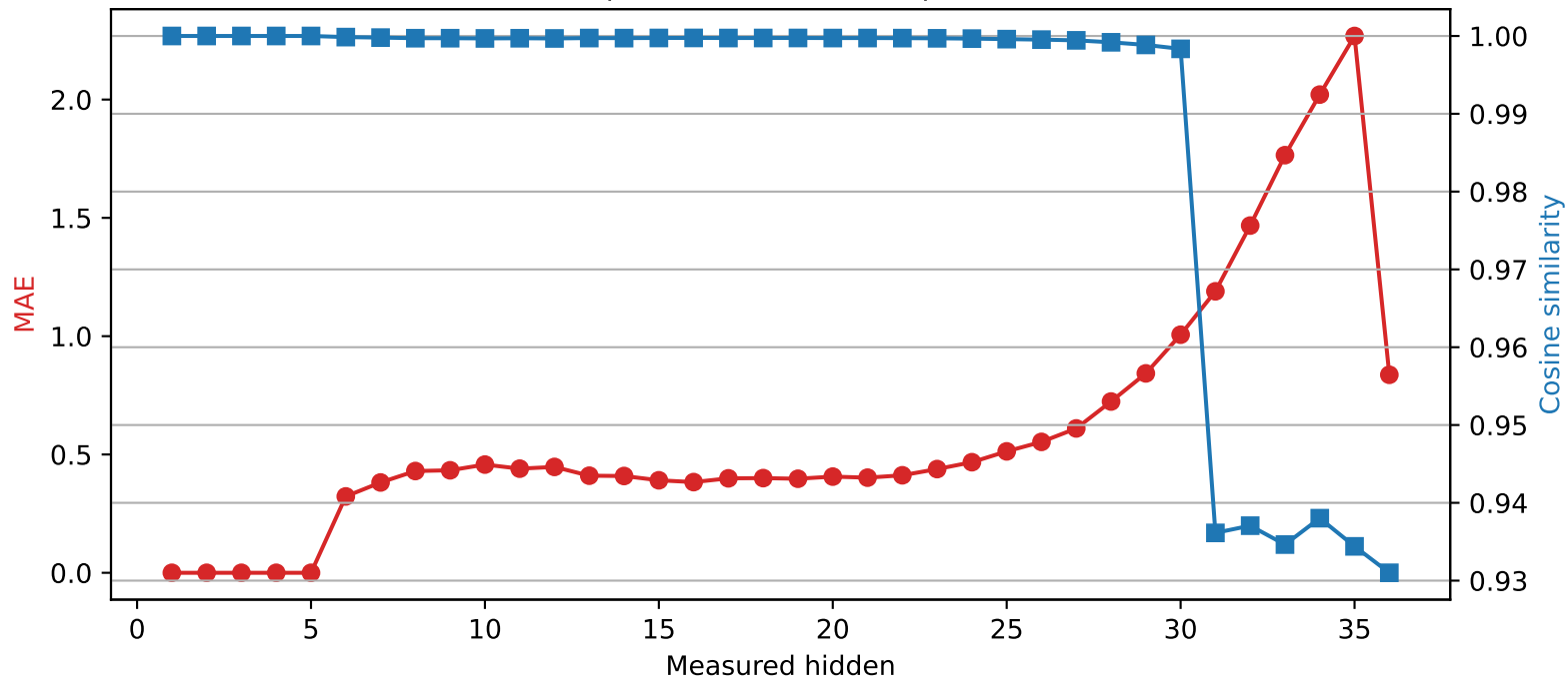
Qwen2.5-3B | Quantized layer 5 | float32 → int4
