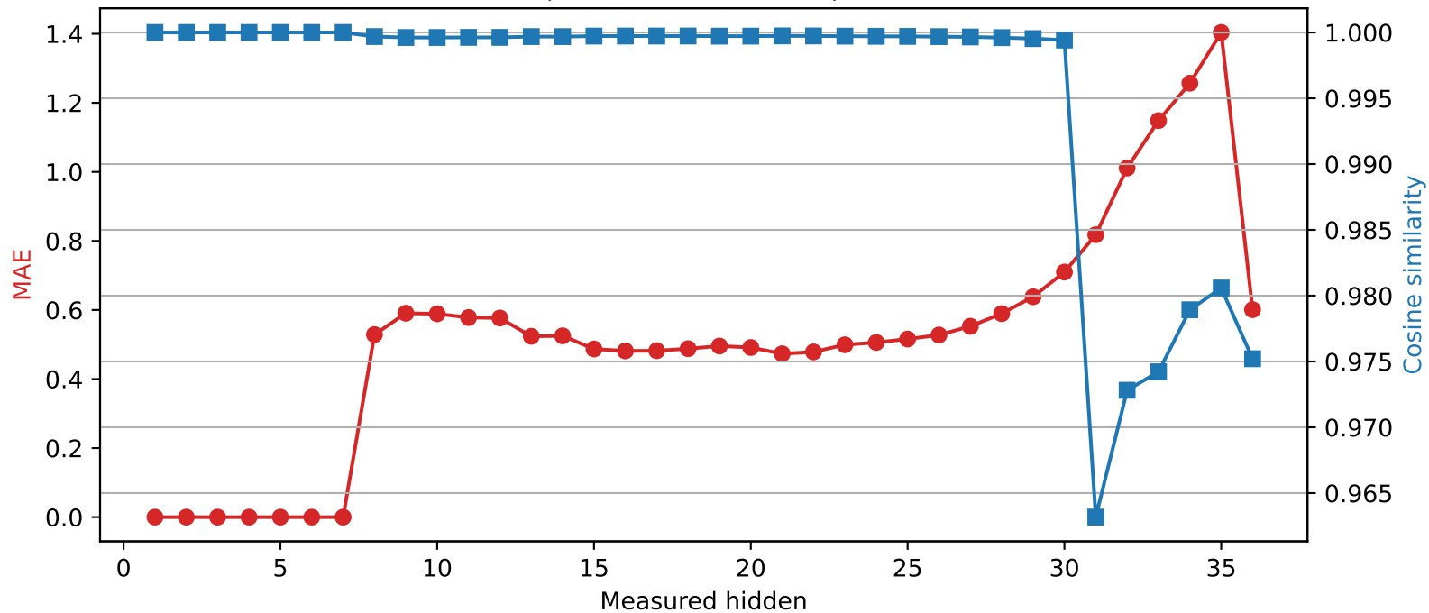
Qwen2.5-3B | Quantized layer 7 | float32 → int4
