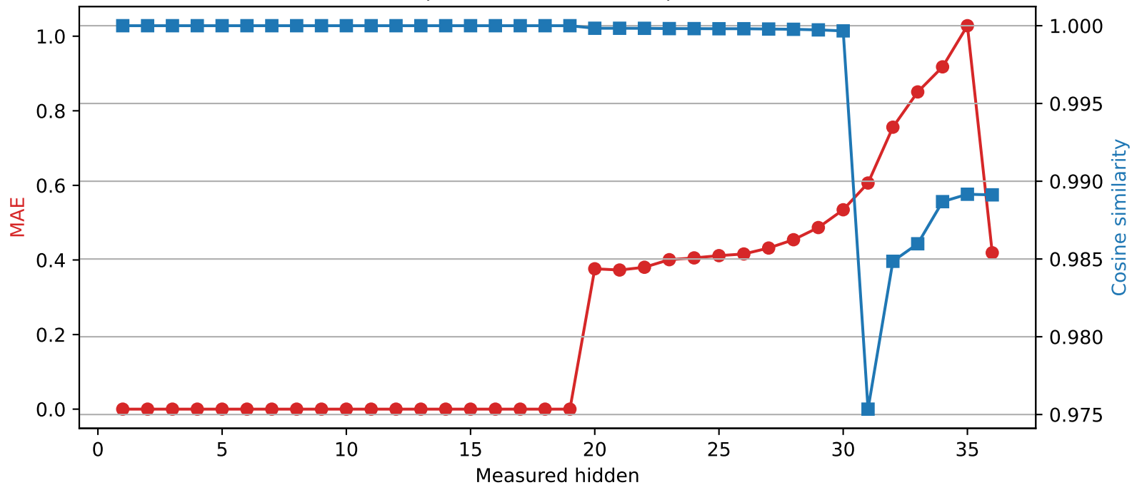
Qwen2.5-3B | Quantized layer 19 | float32 → int4
