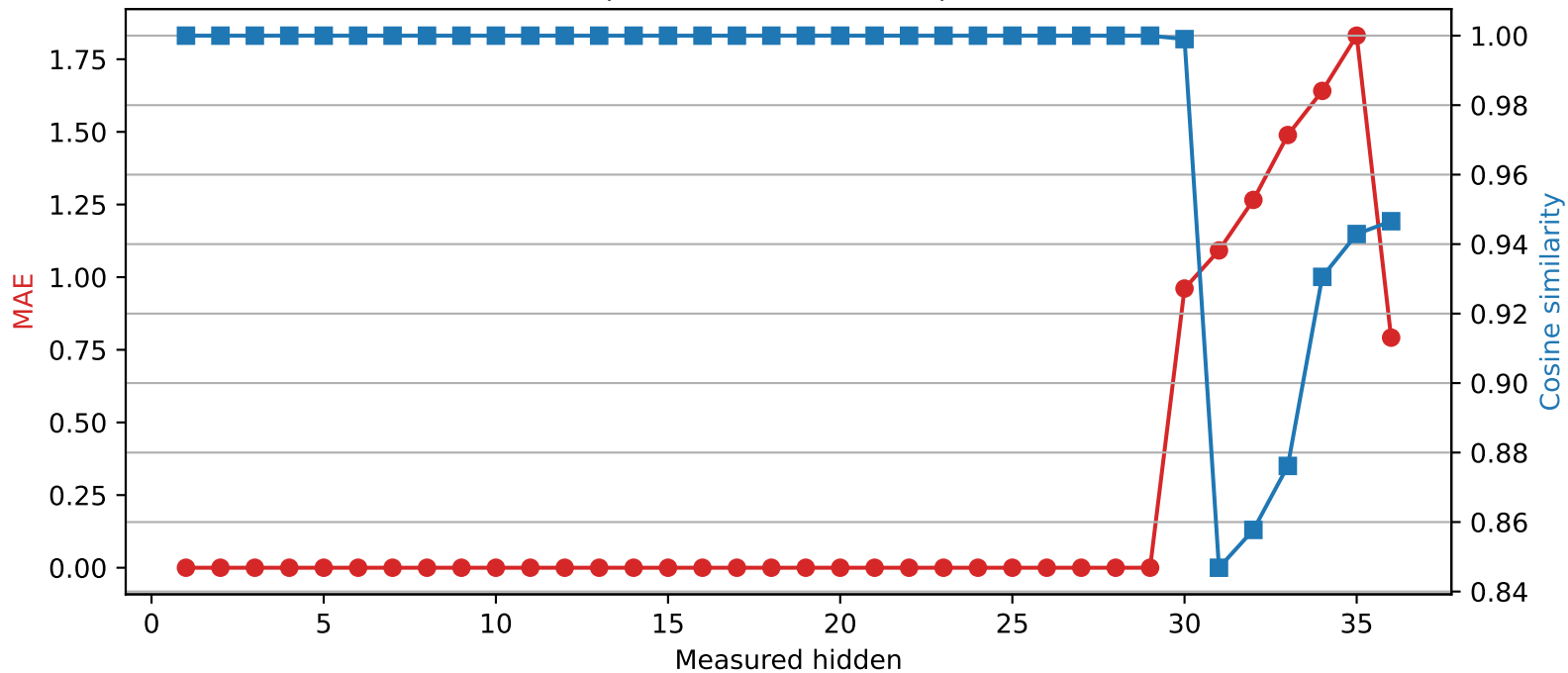
Qwen2.5-3B | Quantized layer 29 | float32 → int4
