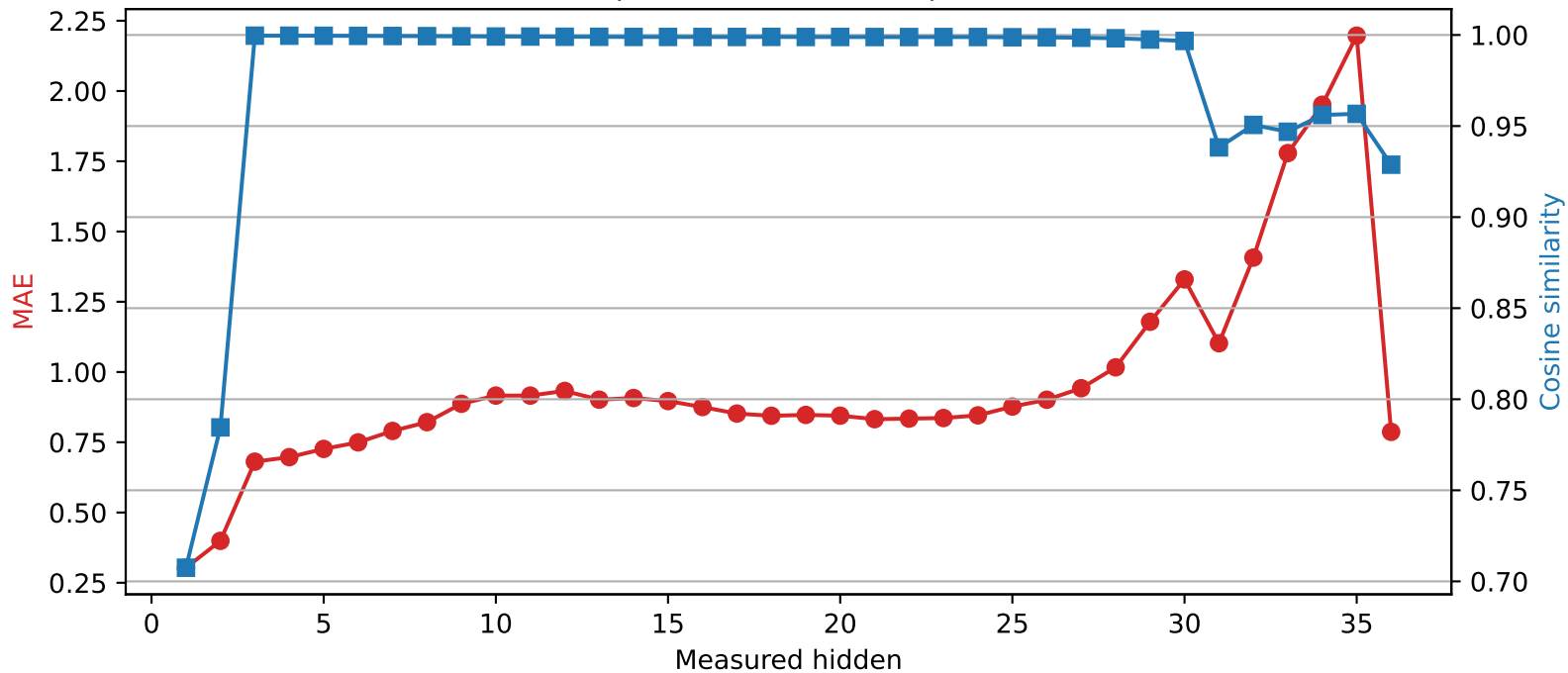
Qwen2.5-3B | Quantized layer 0 | float32 \rightarrow int4
