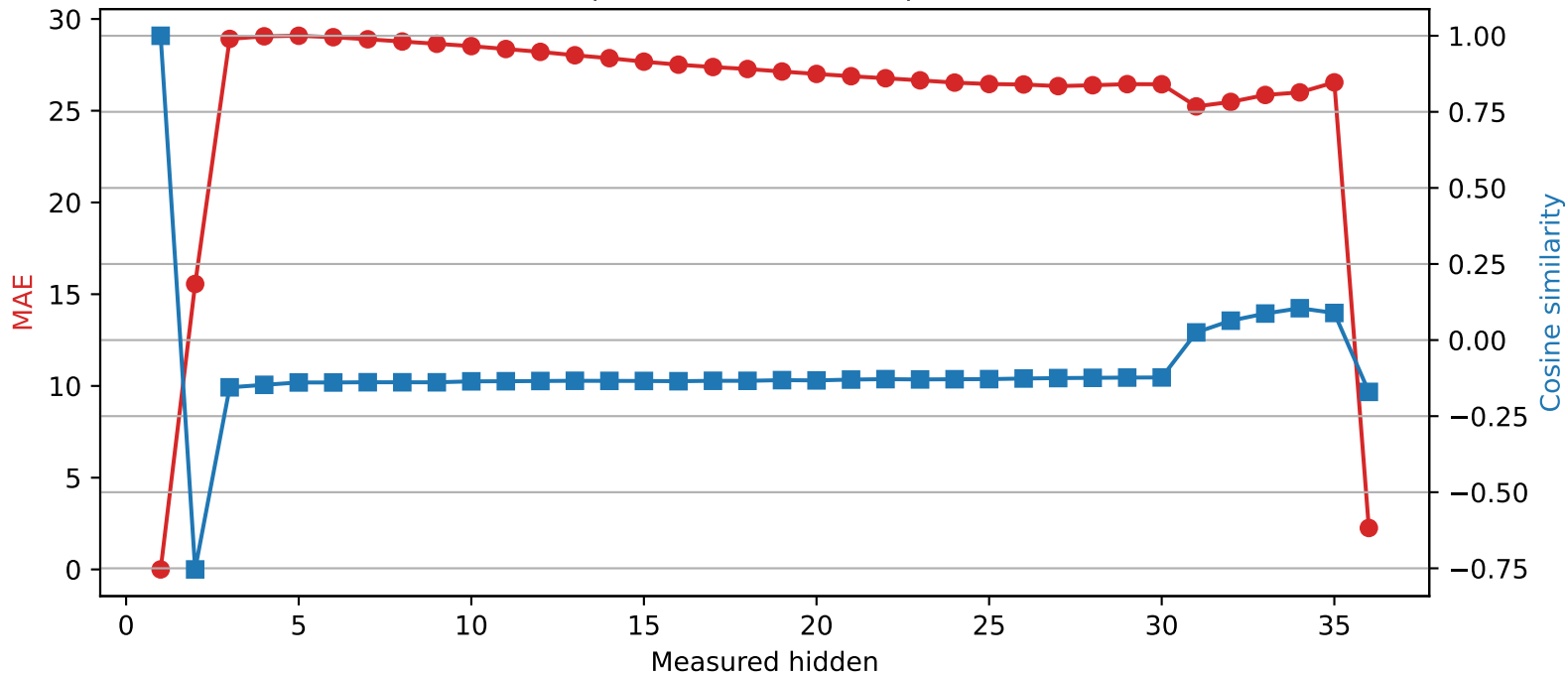
Qwen2.5-3B | Quantized layer 1 | float32 → int4
