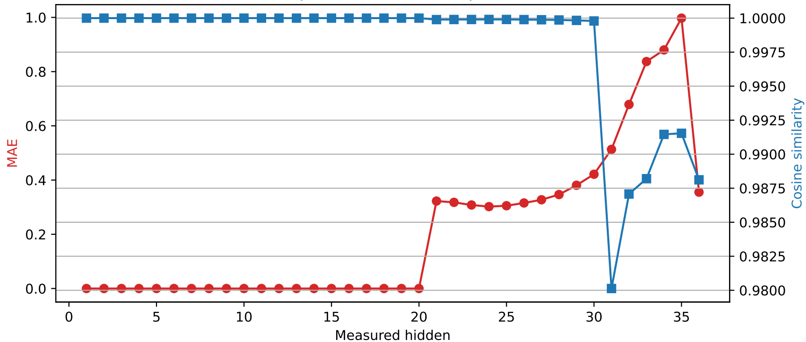
Qwen2.5-3B | Quantized layer 20 | float32 → int4
