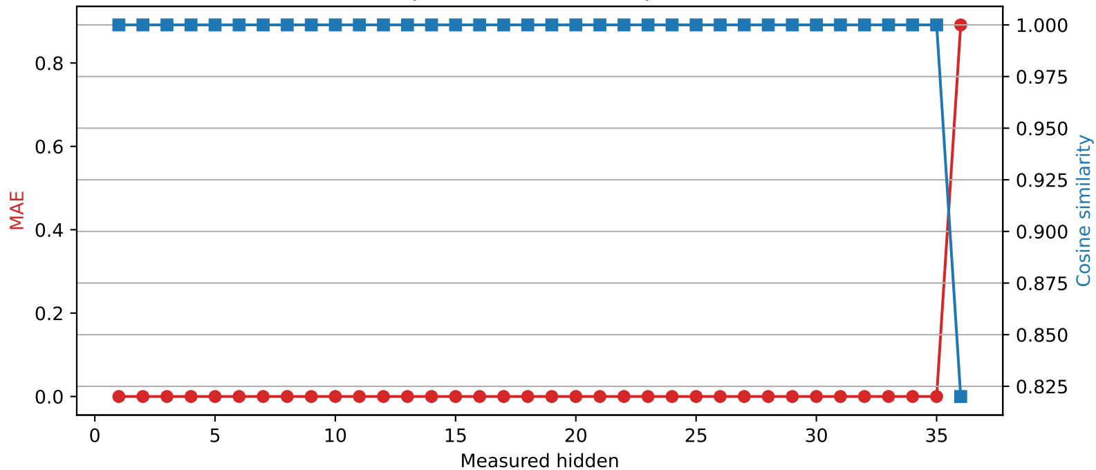
Qwen2.5-3B | Quantized layer 35 | float32 \rightarrow int4
