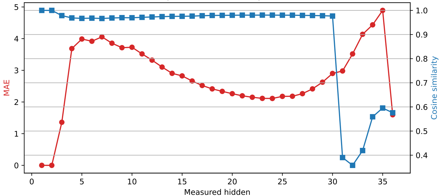
Qwen2.5-3B | Quantized layer 2 | float32 → int4
