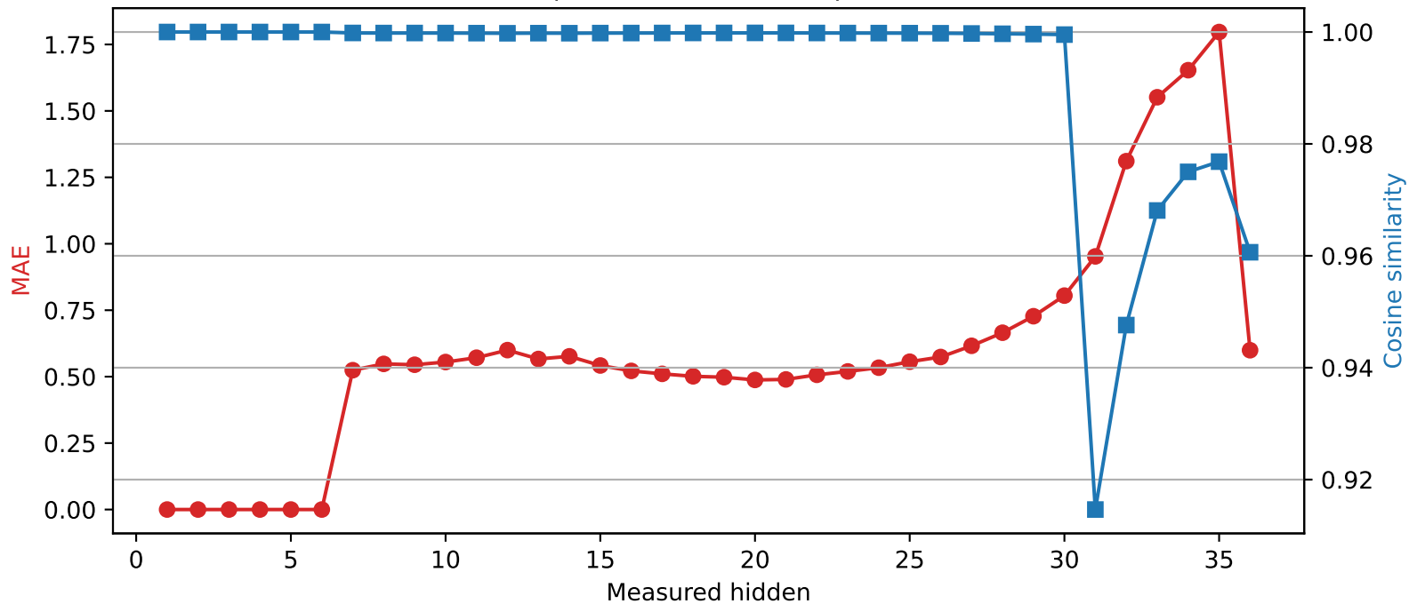
Qwen2.5-3B | Quantized layer 6 | float64 → int4
