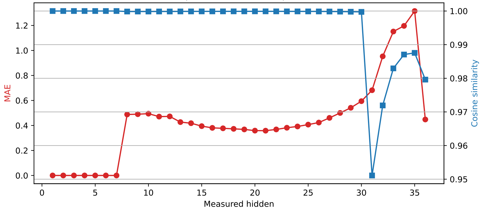
Qwen2.5-3B | Quantized layer 7 | float64 → int4
