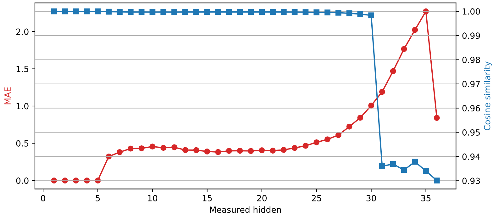
Qwen2.5-3B | Quantized layer 5 | float64 → int4
