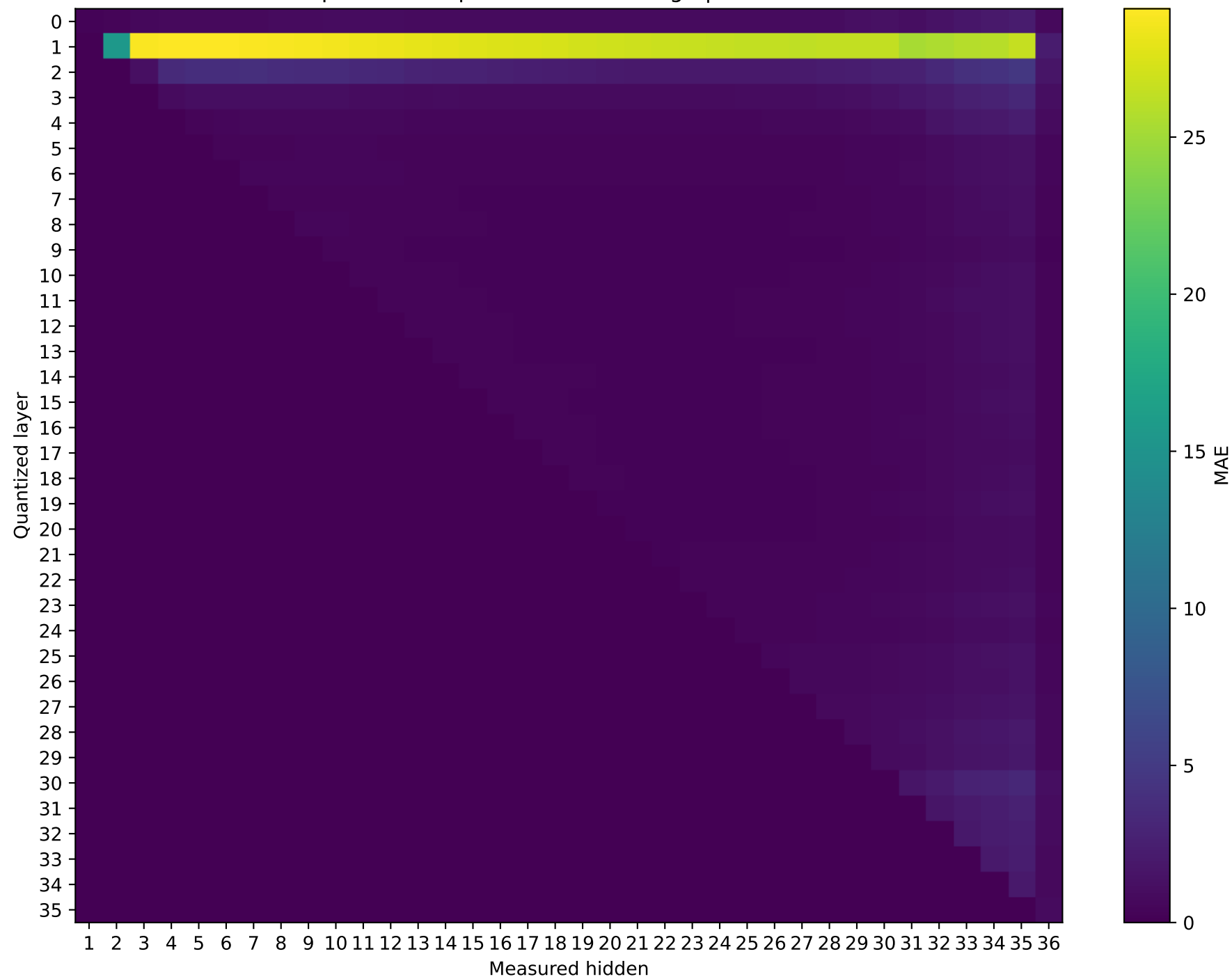
Qwen2.5-3B Prompt 3: MAE representation damage | float64 → int4
