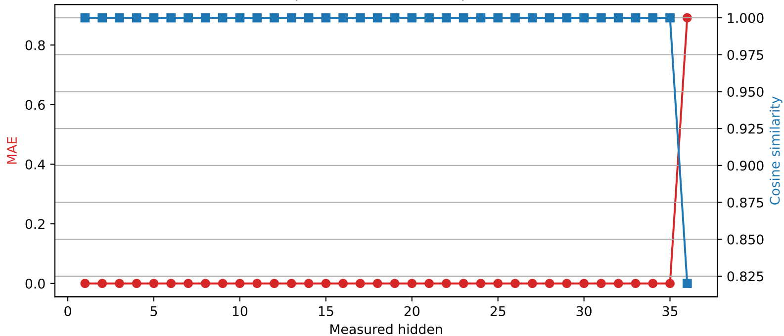
Qwen2.5-3B | Quantized layer 35 | float64 → int4
