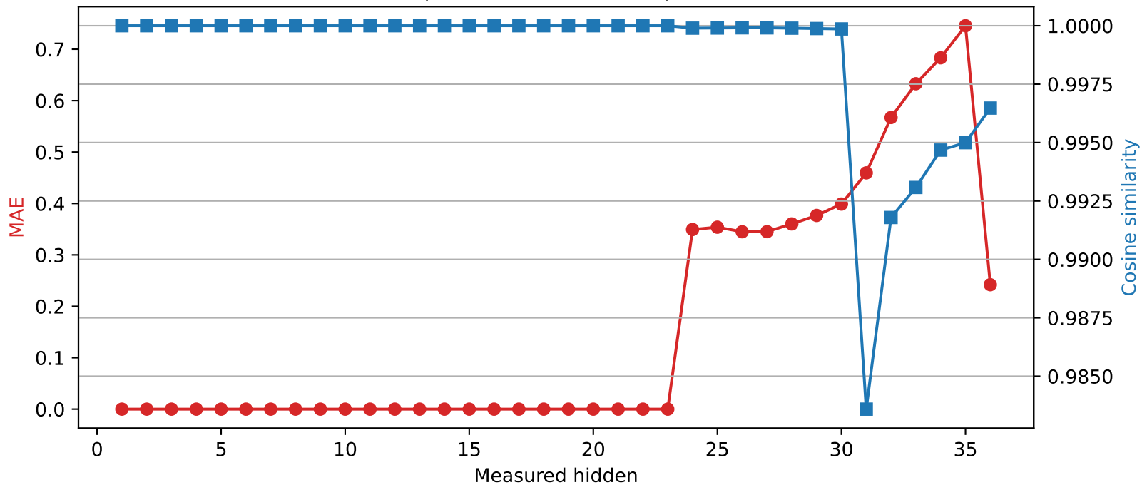
Qwen2.5-3B | Quantized layer 23 | float64 → int4
