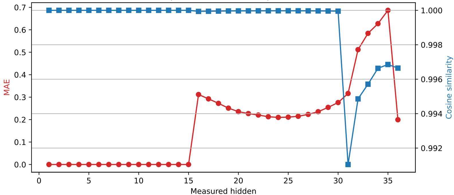
Qwen2.5-3B | Quantized layer 15 | float16 → int2
