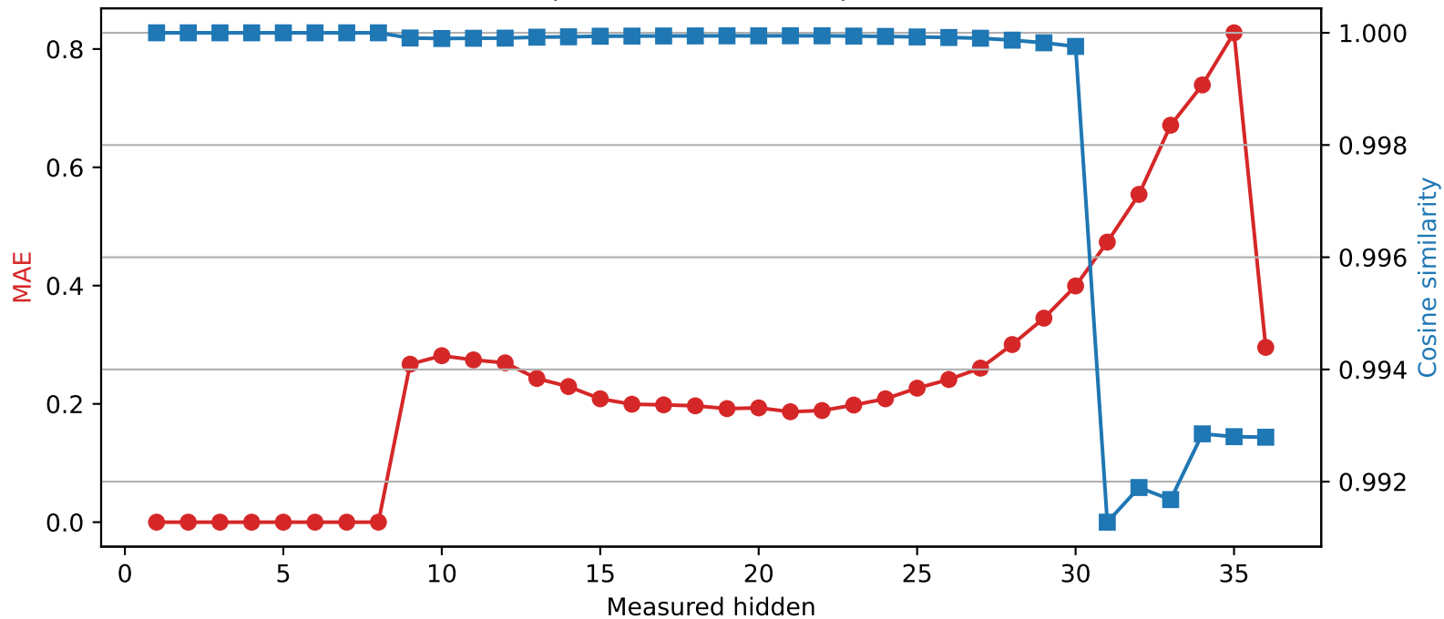
Qwen2.5-3B | Quantized layer 8 | float16 \rightarrow int2
