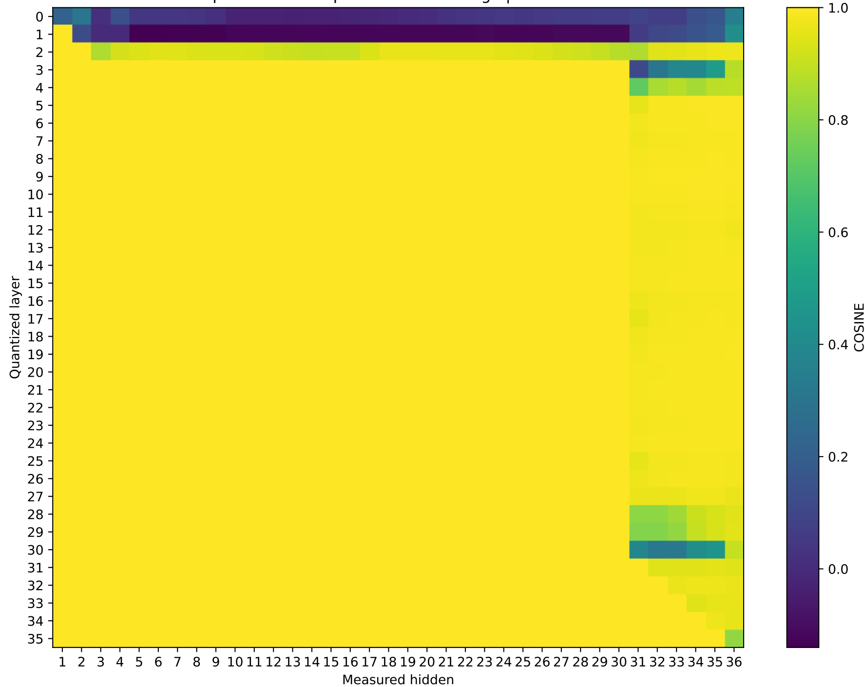
Qwen2.5-3B Prompt 2: cos sim representation damage | float16 \rightarrow int2
