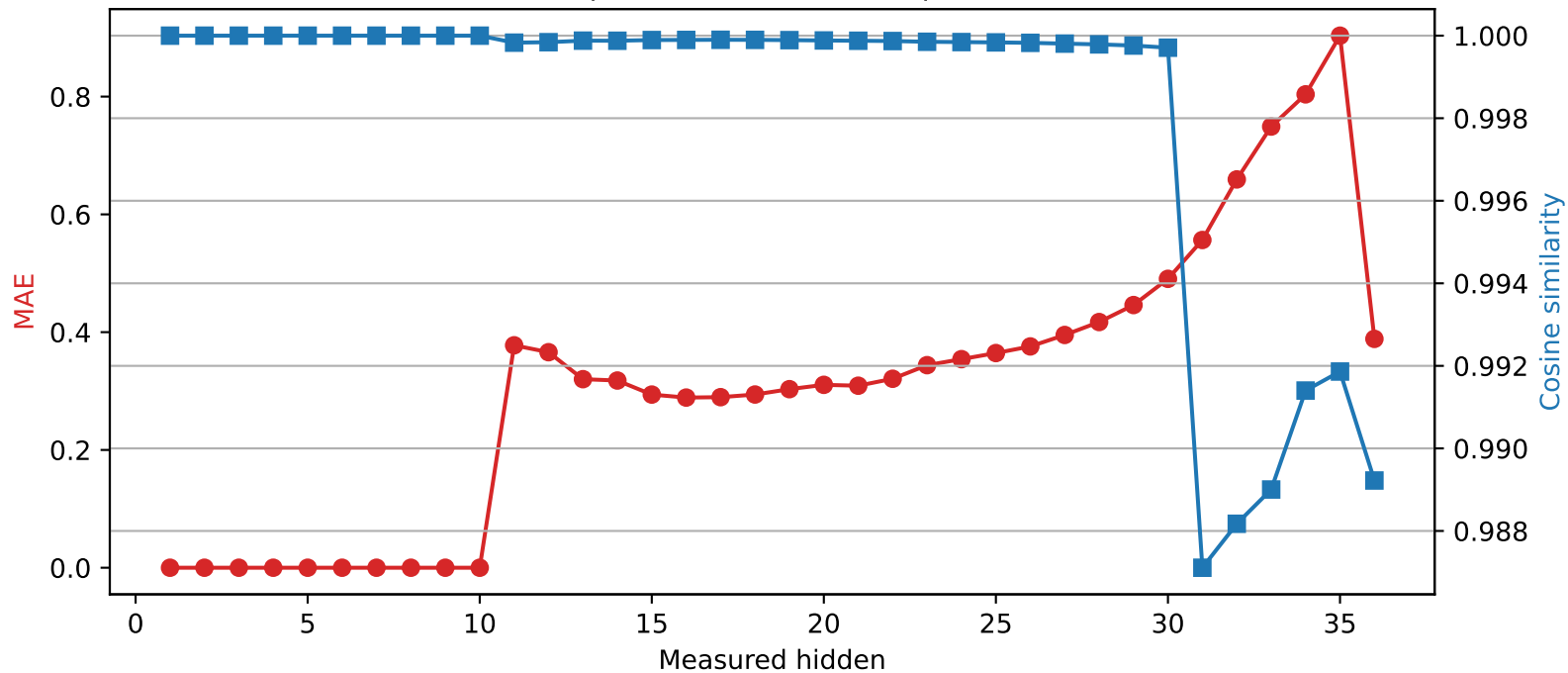
Qwen2.5-3B | Quantized layer 10 | float16 → int2
