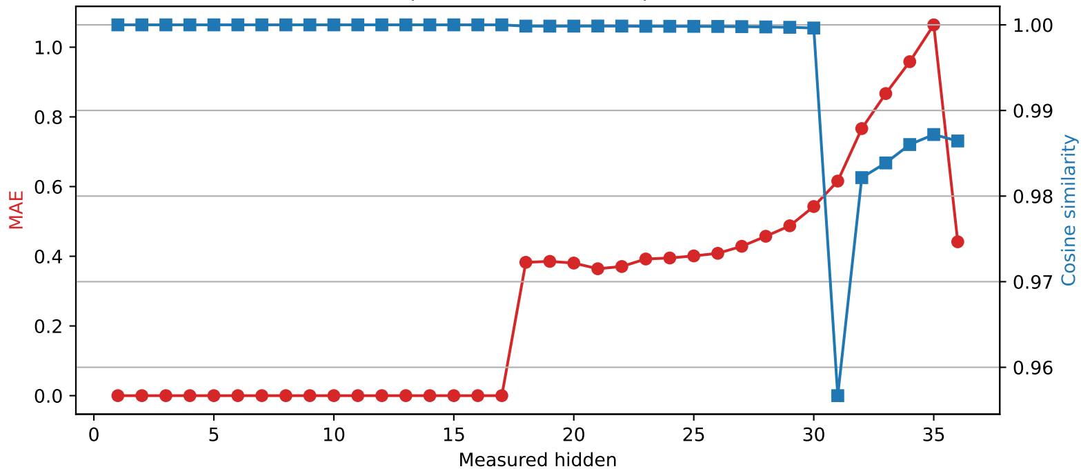
Qwen2.5-3B | Quantized layer 17 | float16 → int2
