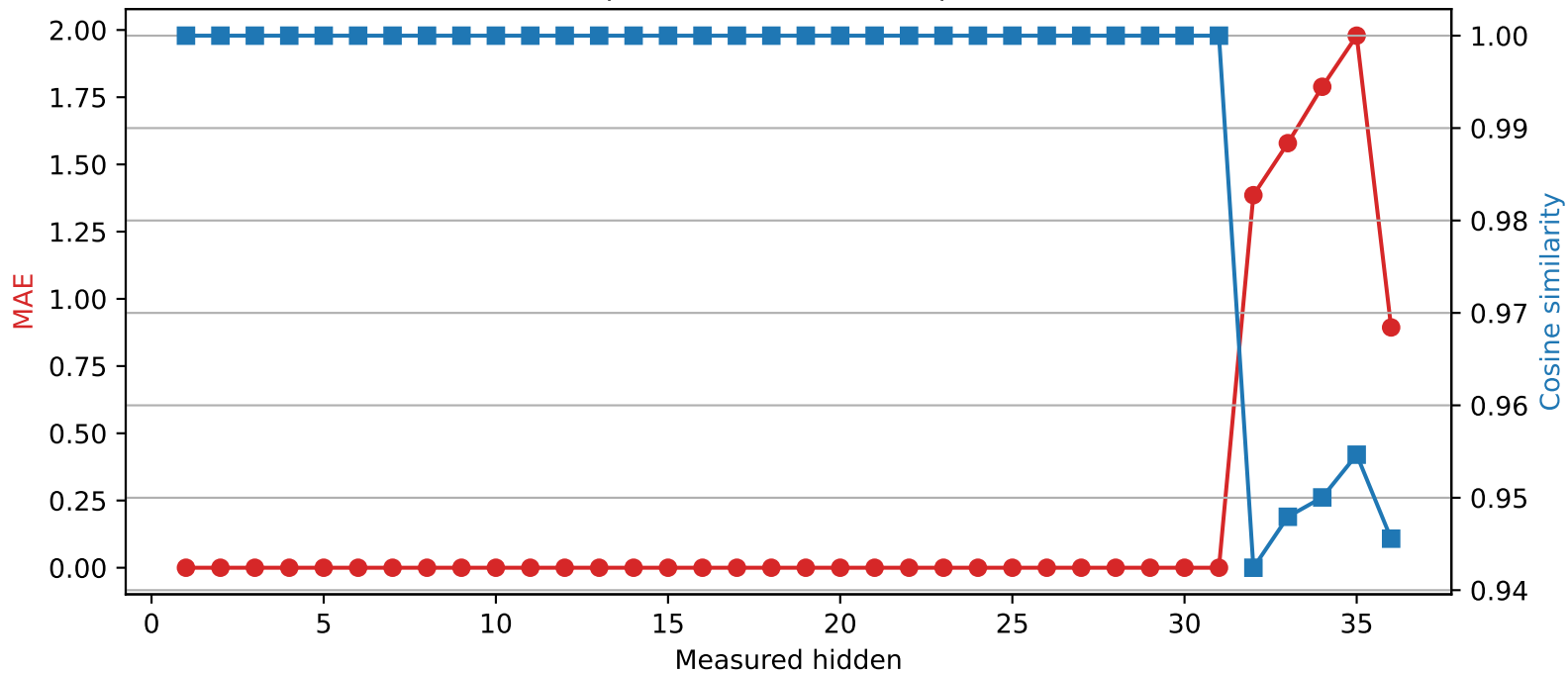
Qwen2.5-3B | Quantized layer 31 | float16 → int2
