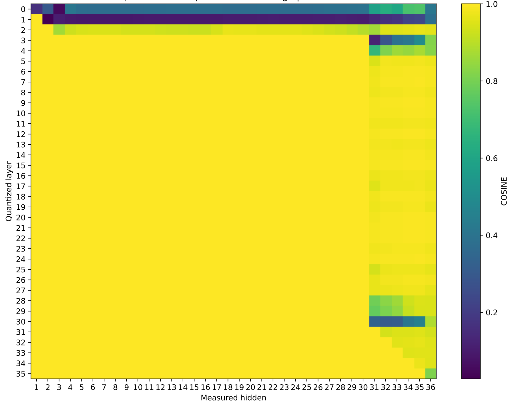
Qwen2.5-3B Prompt 3: cos sim representation damage | float16 → int2
