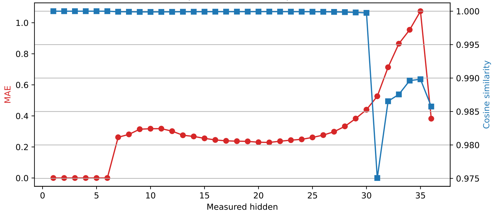
Qwen2.5-3B | Quantized layer 6 | float16 → int2
