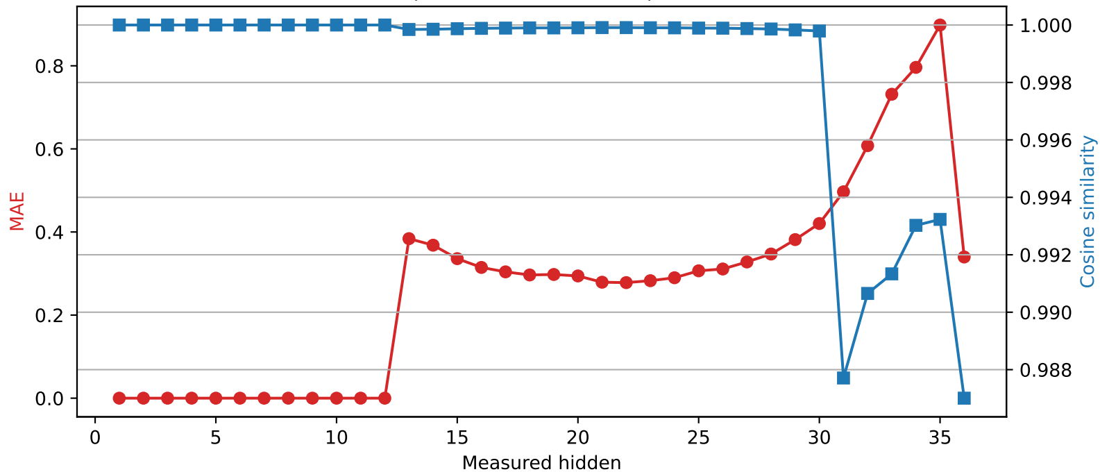
Qwen2.5-3B | Quantized layer 12 | float16 → int2
