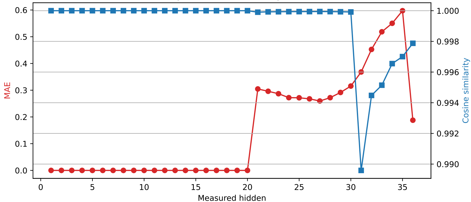
Qwen2.5-3B | Quantized layer 20 | float16 → int2
