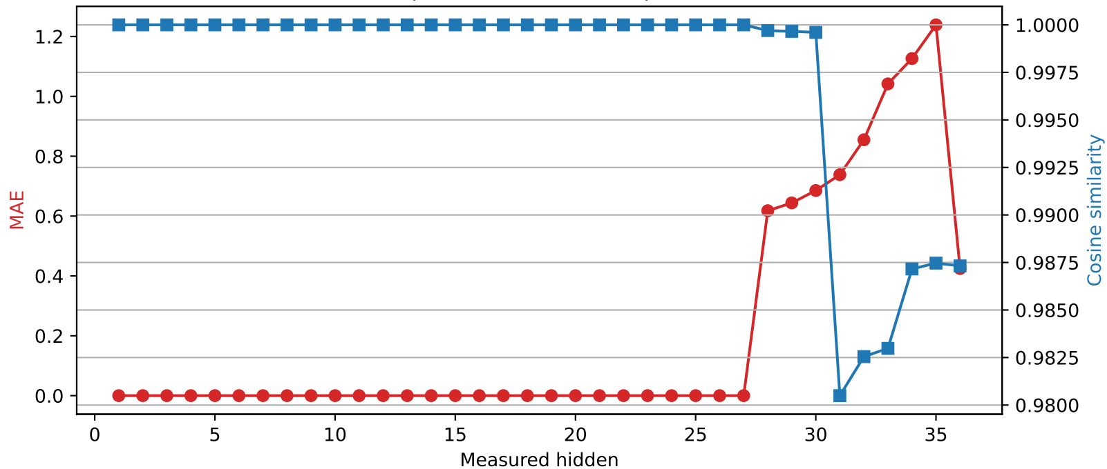
Qwen2.5-3B | Quantized layer 27 | float16 → int2
