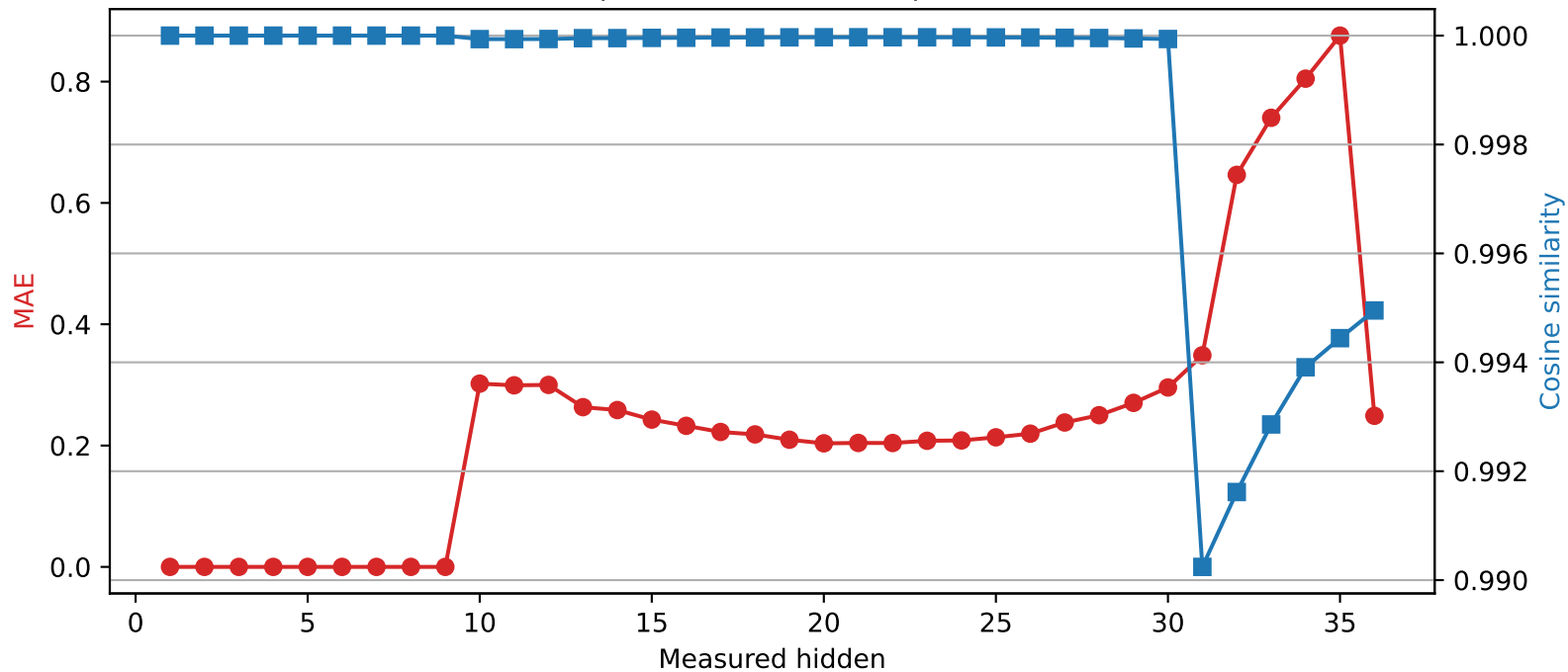
Qwen2.5-3B | Quantized layer 9 | float32 → int2
