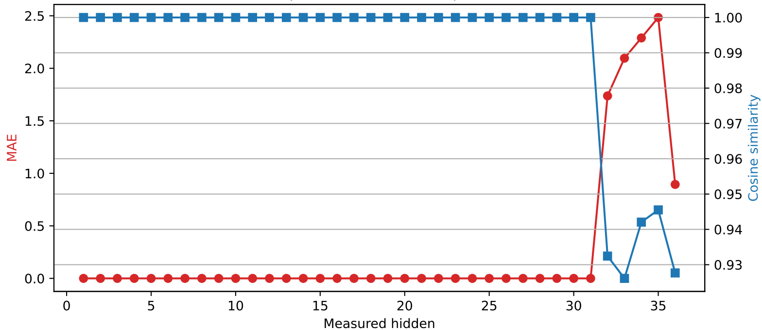
Qwen2.5-3B | Quantized layer 31 | float32 → int2
