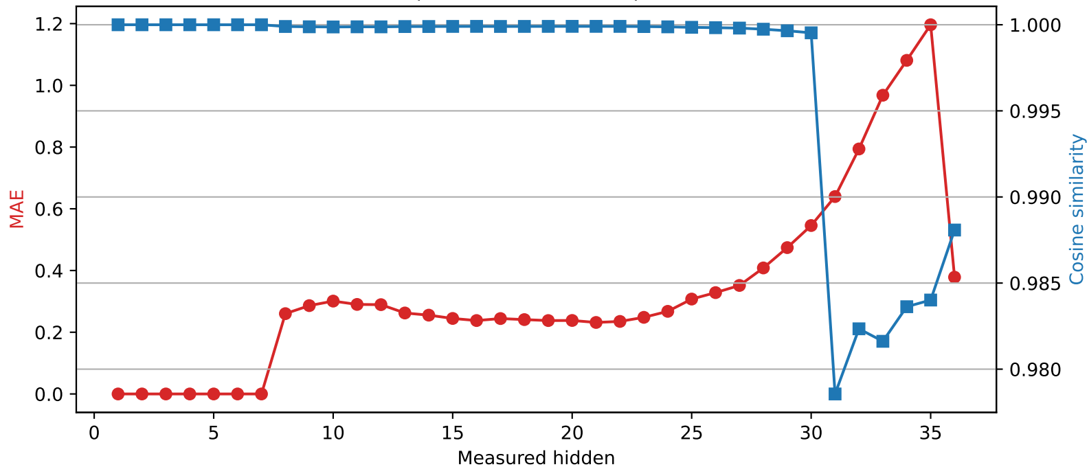
Qwen2.5-3B | Quantized layer 7 | float32 \rightarrow int2
