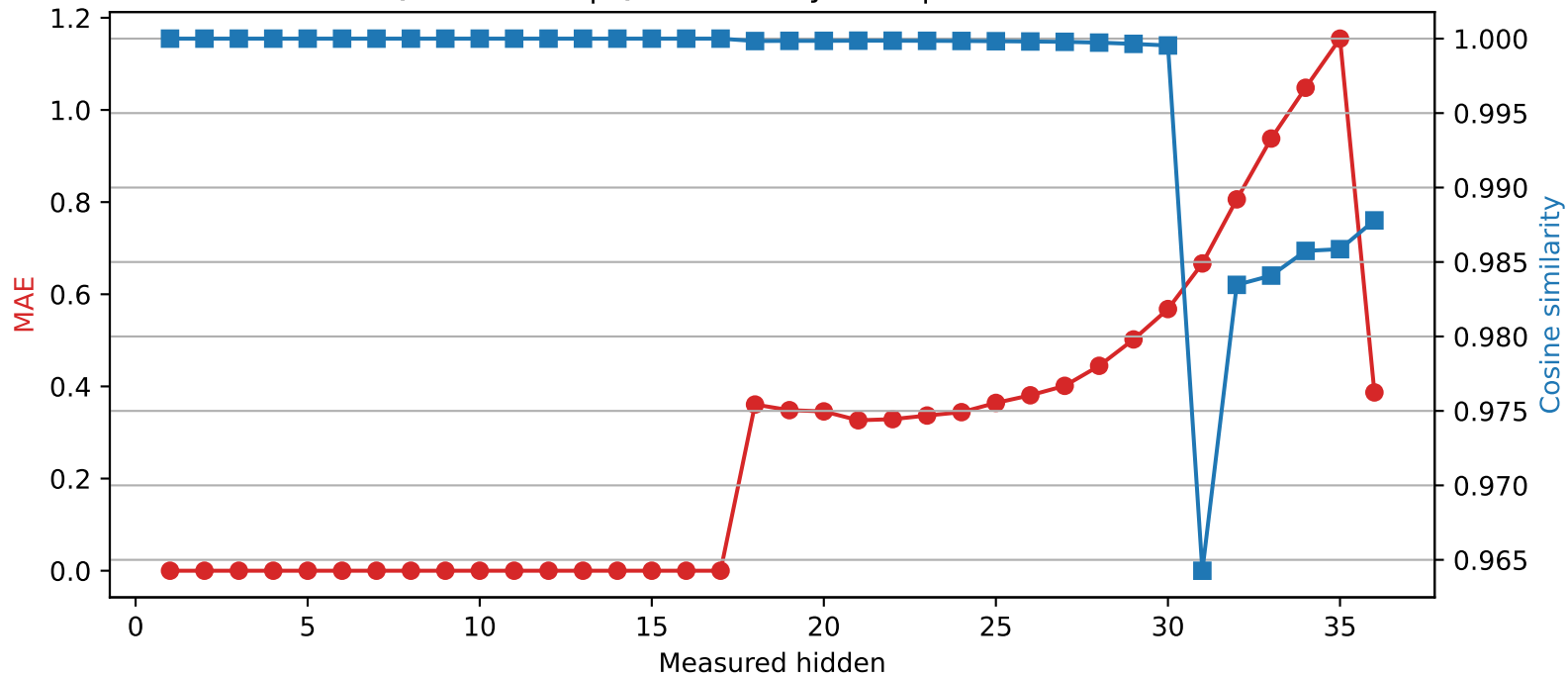
Qwen2.5-3B | Quantized layer 17 | float32 → int2
