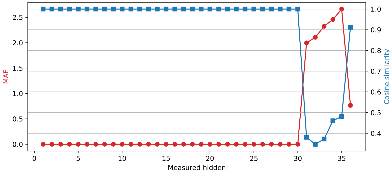
Qwen2.5-3B | Quantized layer 30 | float32 → int2
