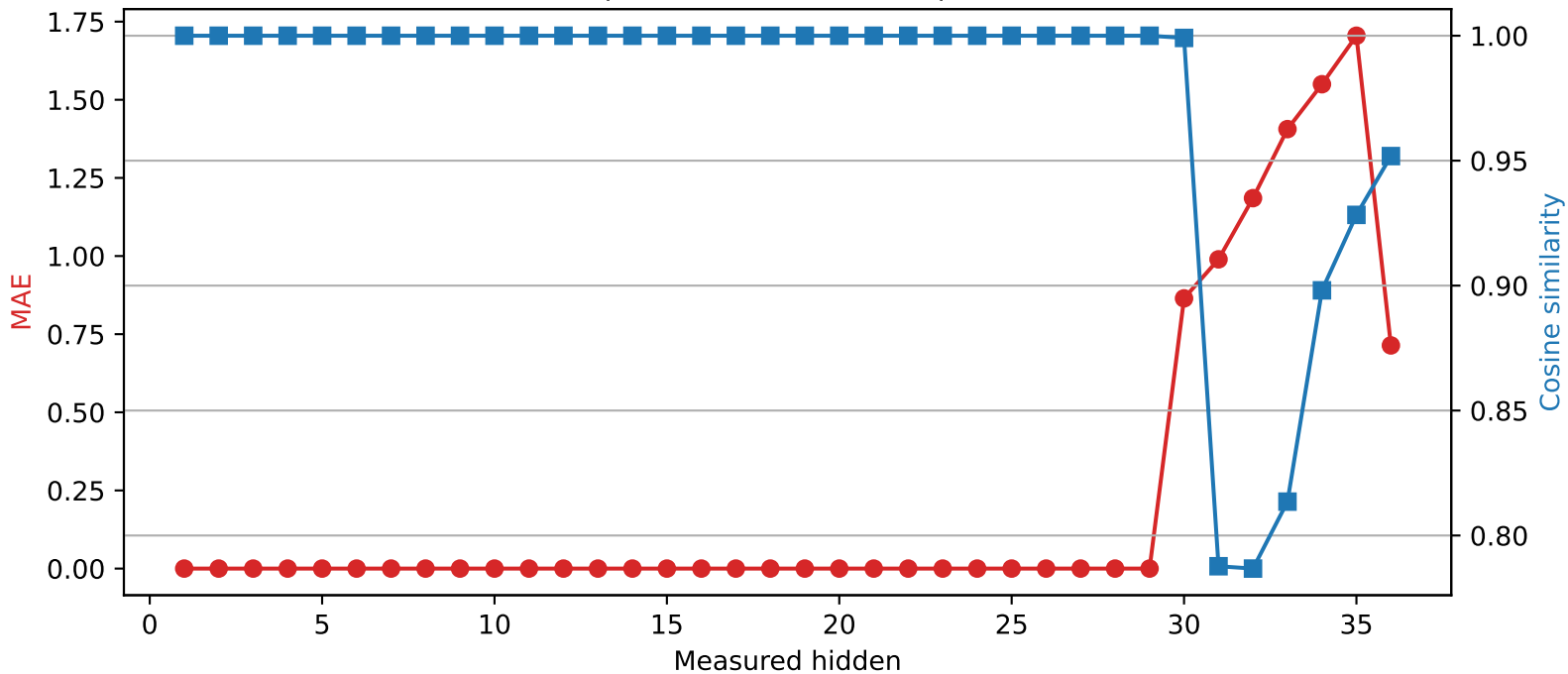
Qwen2.5-3B | Quantized layer 29 | float32 → int2
