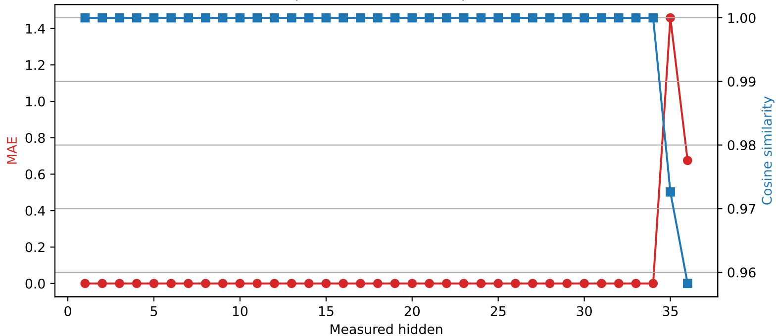
Qwen2.5-3B | Quantized layer 34 | float32 → int2
