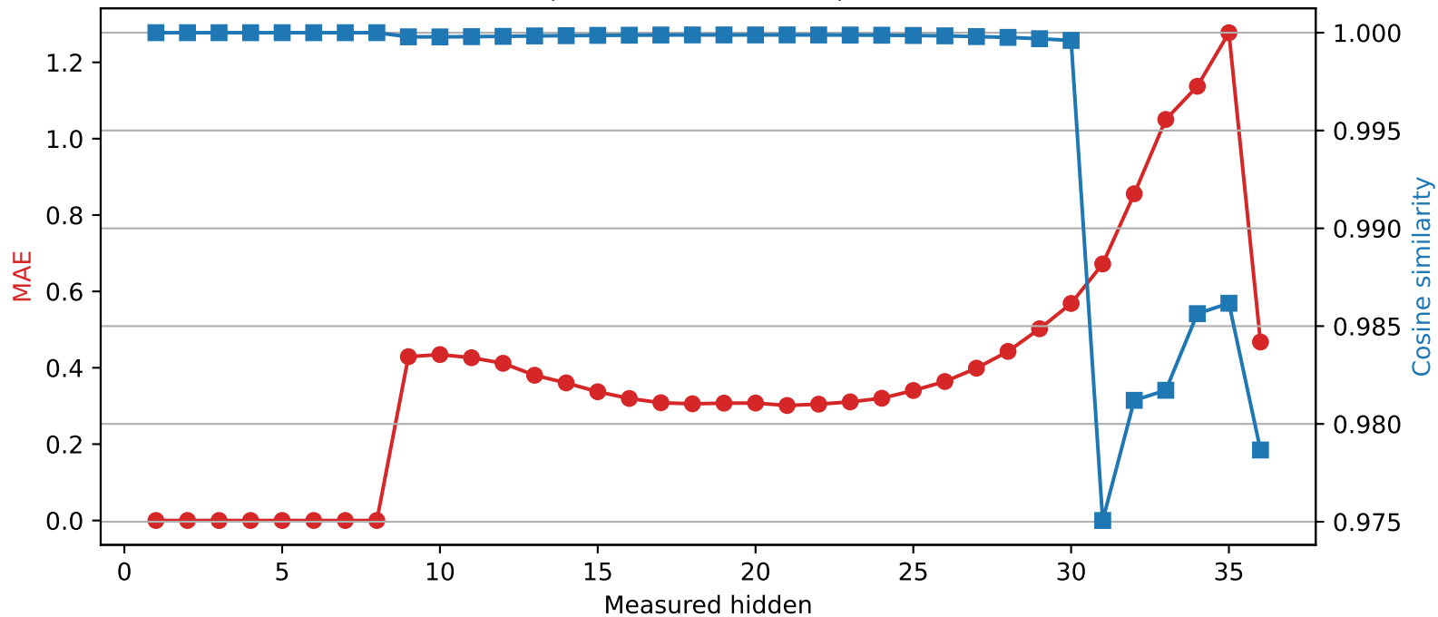
Qwen2.5-3B | Quantized layer 8 | float32 → int2
