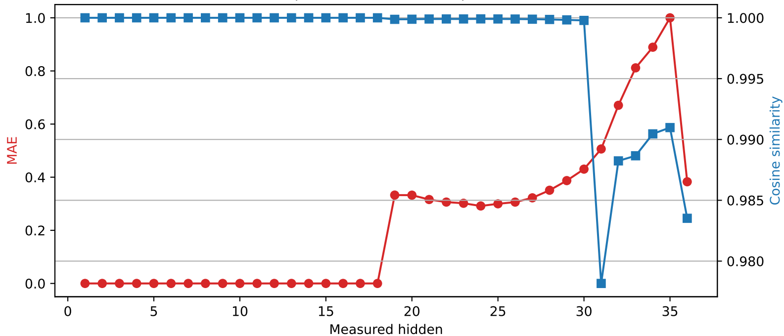
Qwen2.5-3B | Quantized layer 18 | float32 → int2
