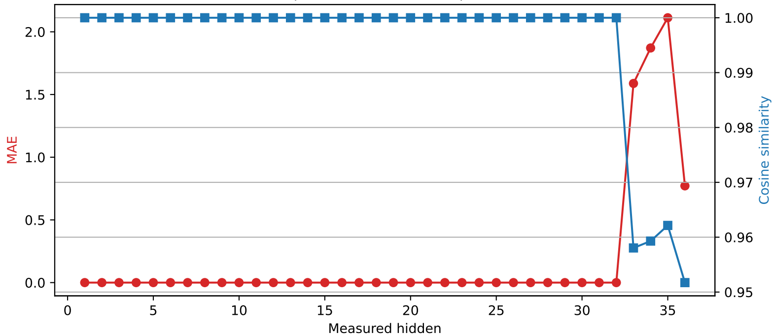
Qwen2.5-3B | Quantized layer 32 | float32 → int2
