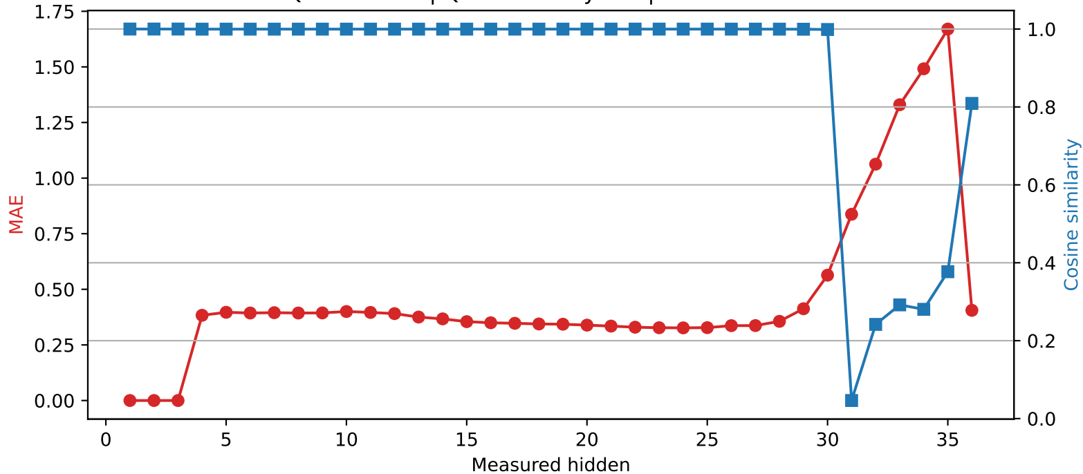
Qwen2.5-3B | Quantized layer 3 | float32 \rightarrow int2
