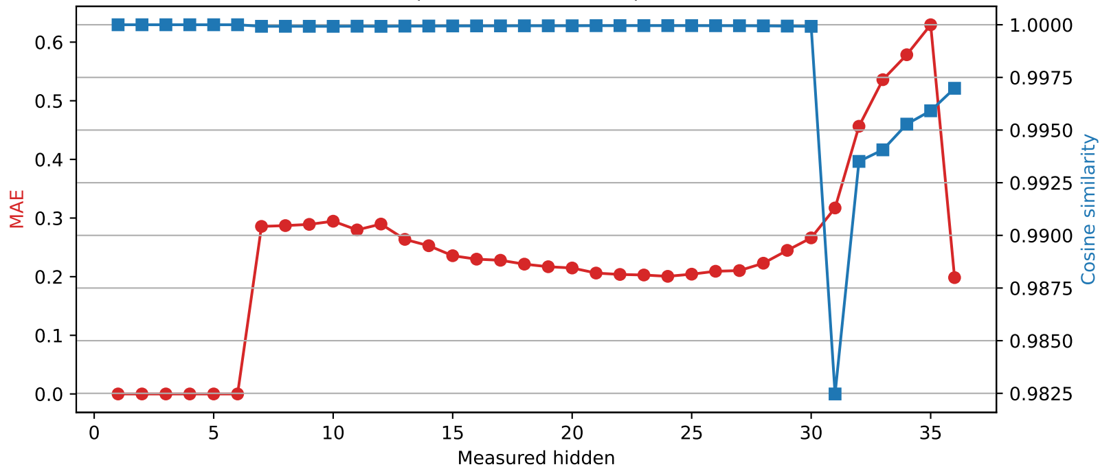
Qwen2.5-3B | Quantized layer 6 | float32 → int2
