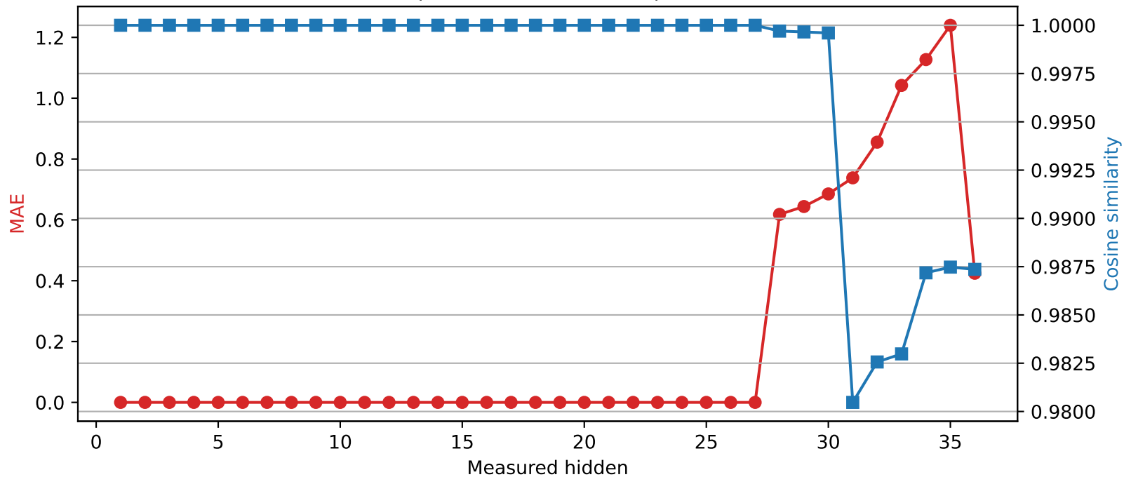
Qwen2.5-3B | Quantized layer 27 | float32 → int2
