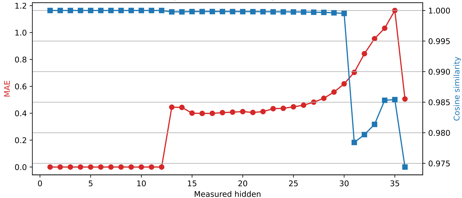
Qwen2.5-3B | Quantized layer 12 | float64 → int2
